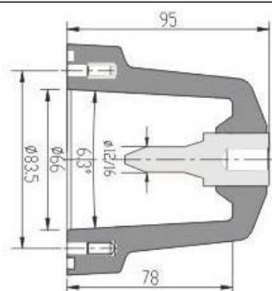
15kV I Bus-bar socket
