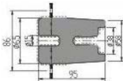
15kV I plug
